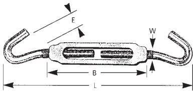
Extruded aluminum bodies with zinc chromate steel hooks
