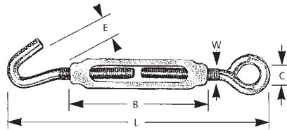
Extruded aluminum bodies with zinc chromate steel eyes and hooks
